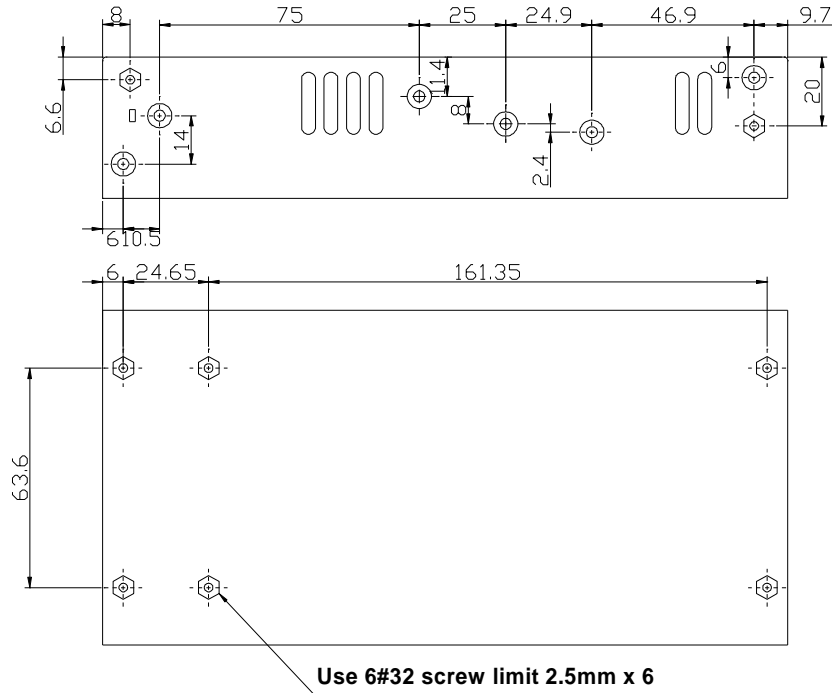
The mechanical drawing of bottom enclosure ( and spec of fixed screws ):
