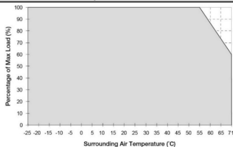
Temperature/Load
