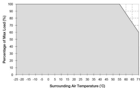
Temperature/Load
