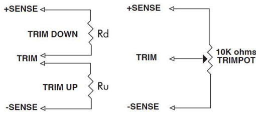
AER75-XXS05 Trim Table
