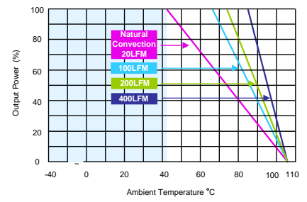
AER75-72S05, AER75-110S05 Derating Curve with Heatsink
