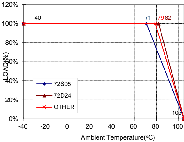
Typical Derating curve for Natural Convection
