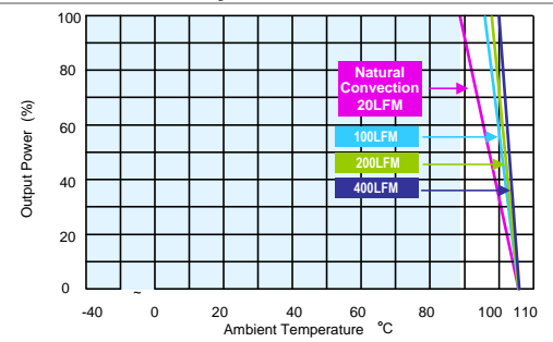
AER10-24S12, AER10-24D12, AER10-48S24, AER10-110D12 AER10-110D15 Derating Curve with Heatsink
