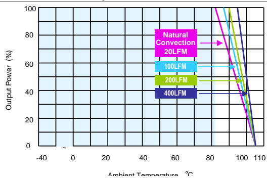
AER10-24S05 Derating Curve without Heatsink
