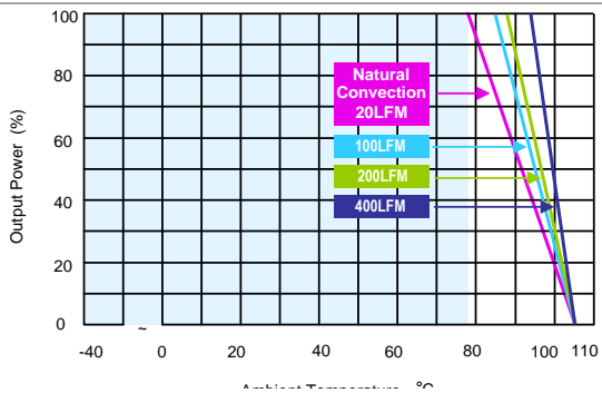
AER10-110S05 Derating Curve without Heatsink
