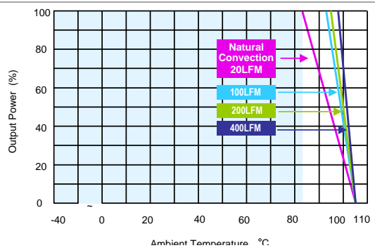
AER10-110S05 Derating Curve with Heatsink
