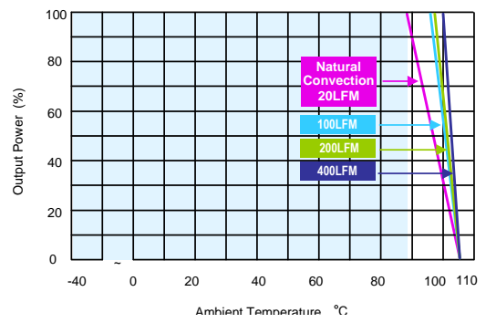
AER10-48S05, AER10-110S12, AER10-110S15, AER10-110S24 Derating Curve with Heatsink
