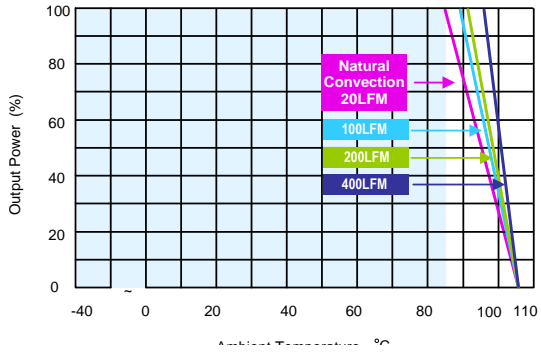
AER10-48S05, AER10-110S12, AER10-110S15, AER10-110S24 Derating Curve without Heatsink
