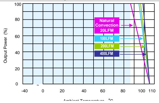
AER10-24S05 Derating Curve with Heatsink
