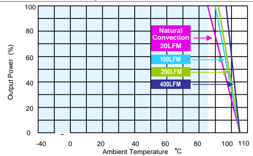
AER10-24S12, AER10-24D12, AER10-48S24, AER10-110D12 AER10-110D15 Derating Curve without Heatsink
